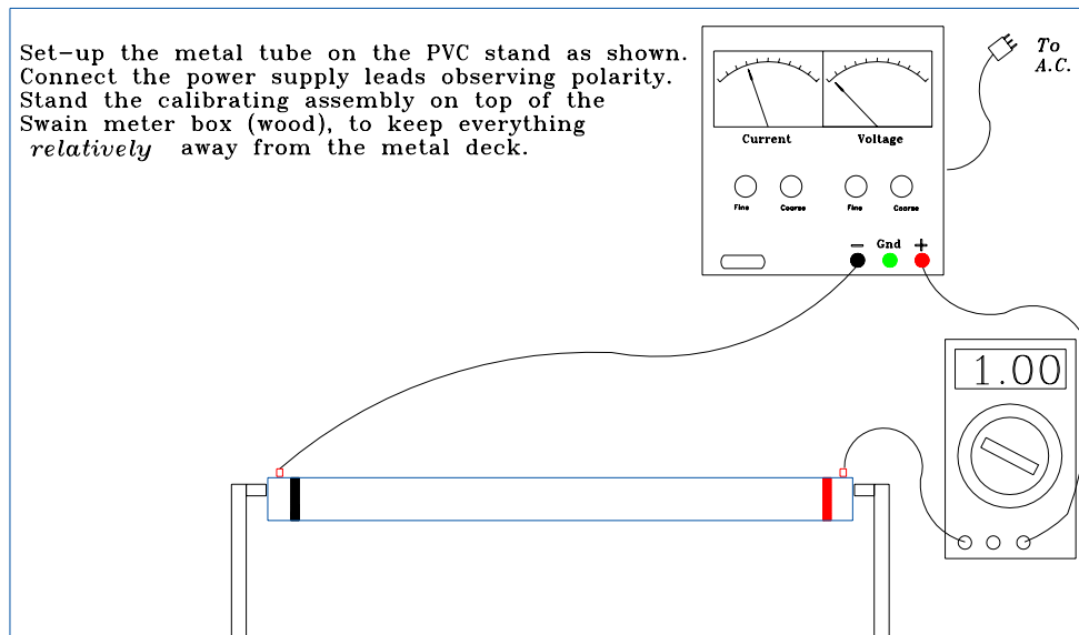
Fig.3 Calibration Set-Up
